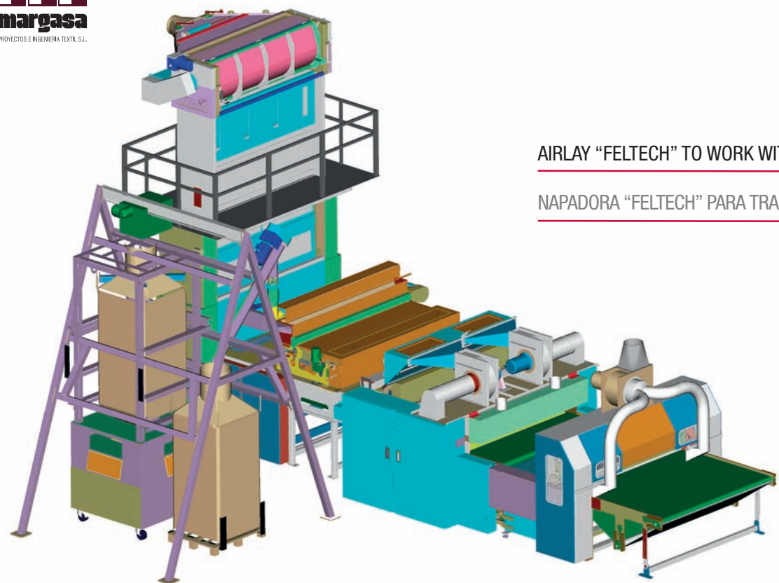
AIRLAY "FELTECH" 2500 MM. WORKING WIDTH WITH AUTOLEVELER FEEDER CNA AND RESIN DISTRIBUTOR
